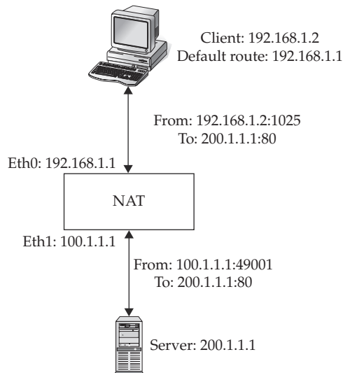
Figure 13-1. Using SNAT on a connection
