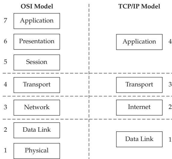
Figure 11-3. The OSI reference model and the TCP/IP model
